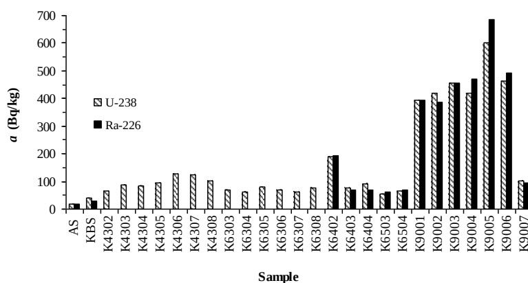
Figure 2. Samples with elevated ^{238}\text{U} and/or ^{226}\text{Ra} massic activities in the Kaštela Bay sediments; massic activities in the AS and KBS are given for comparison
