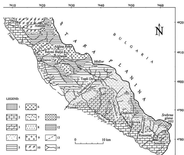
Figure 2. Geological map of Stara Planina in the Serbian territory [2]
