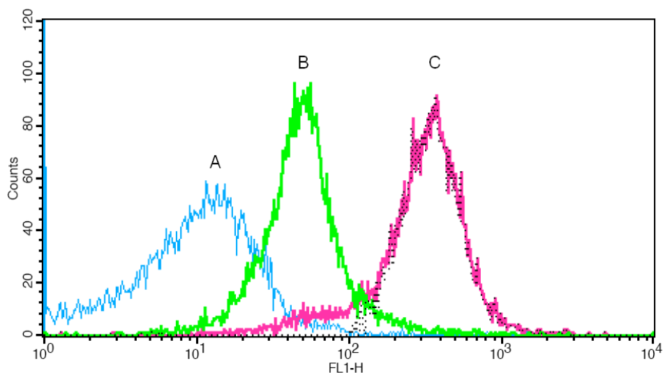
Figure 1. The FL1-H histograms of the FITC signal of the antibody labelled \gamma -phosphorylated H2AX histones that indirectly represent DNA double strand breaks. Line A – non-labelled control; Line B – labelled vehicle control; Line C – labelled 4 Gy irradiated blood sample.
